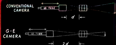
FIG. 1—TWICE THE BACK FOCAL TRAVEL
